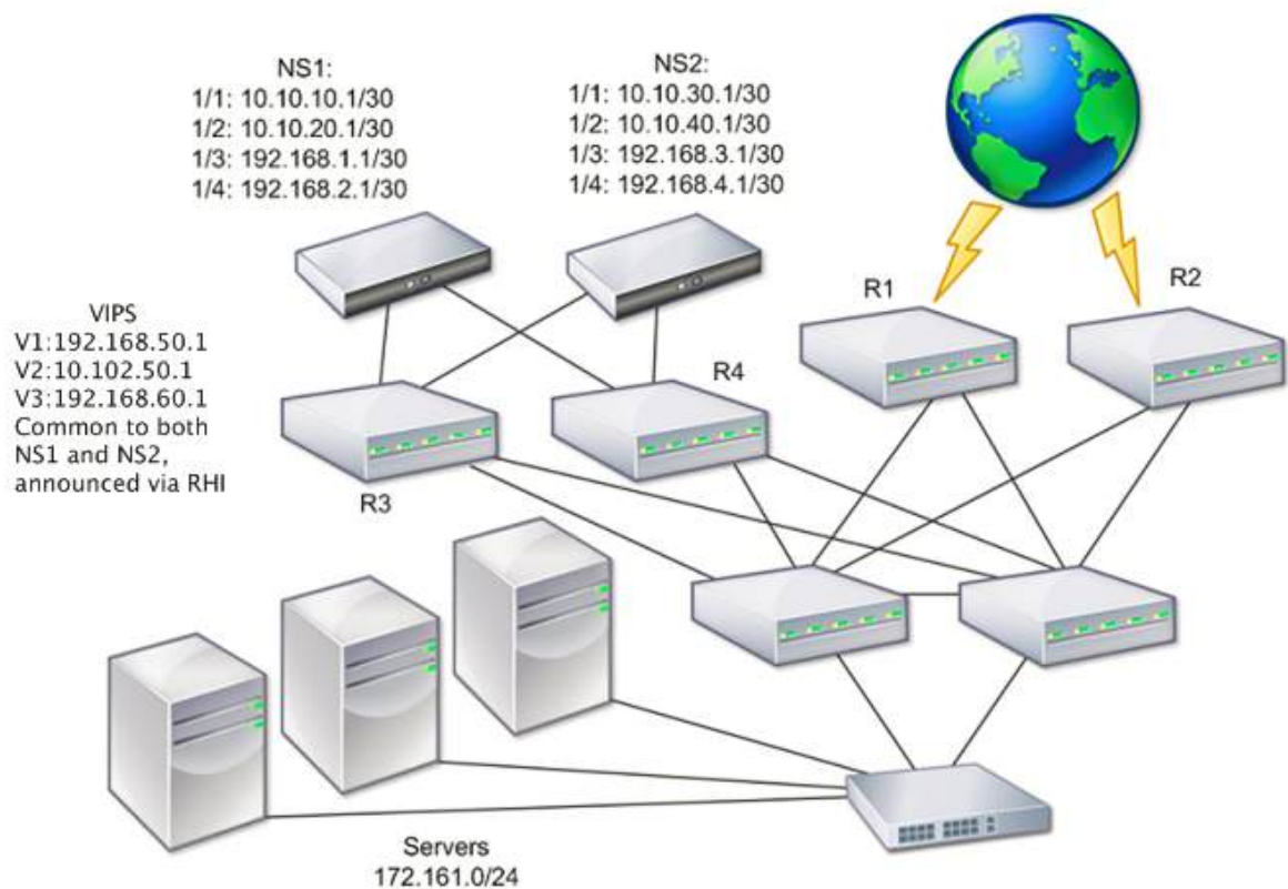
Figure 1. High Availability over a Routed Network
